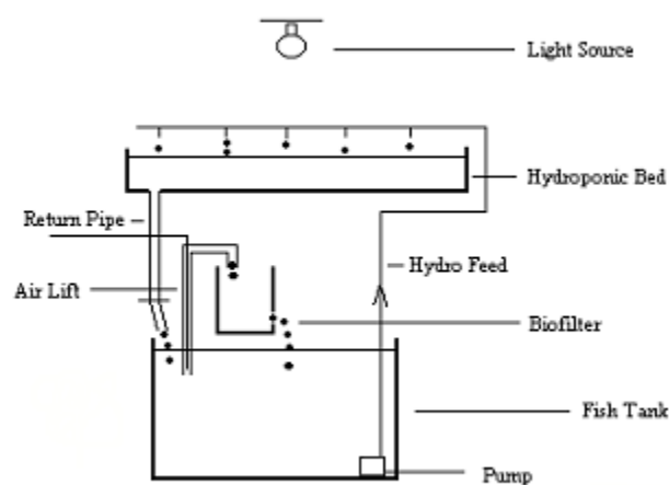
Figure 1: Schematic representation of a single Aquaponic test unit.
